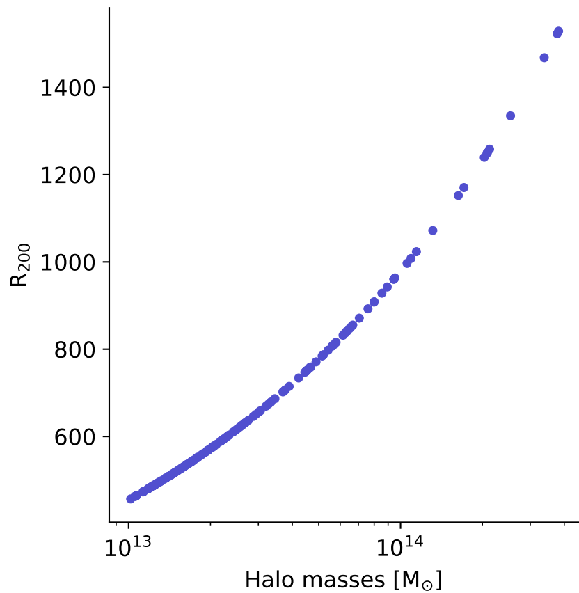
Masses and R_{200} of total sample
