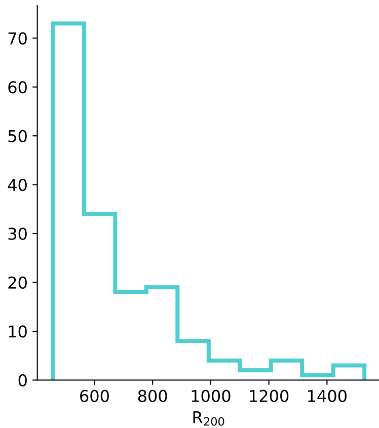
Masses and R_{200} of total sample
